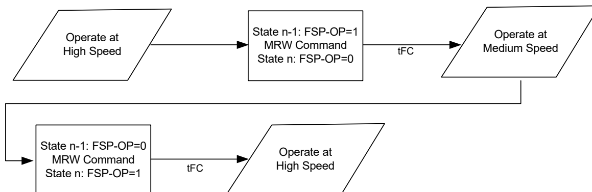
Figure - Switching between two trained Frequency Set Points
