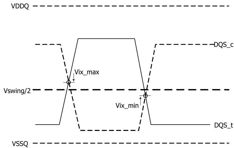
Figure - DQS input crosspoint voltage (Vix)
