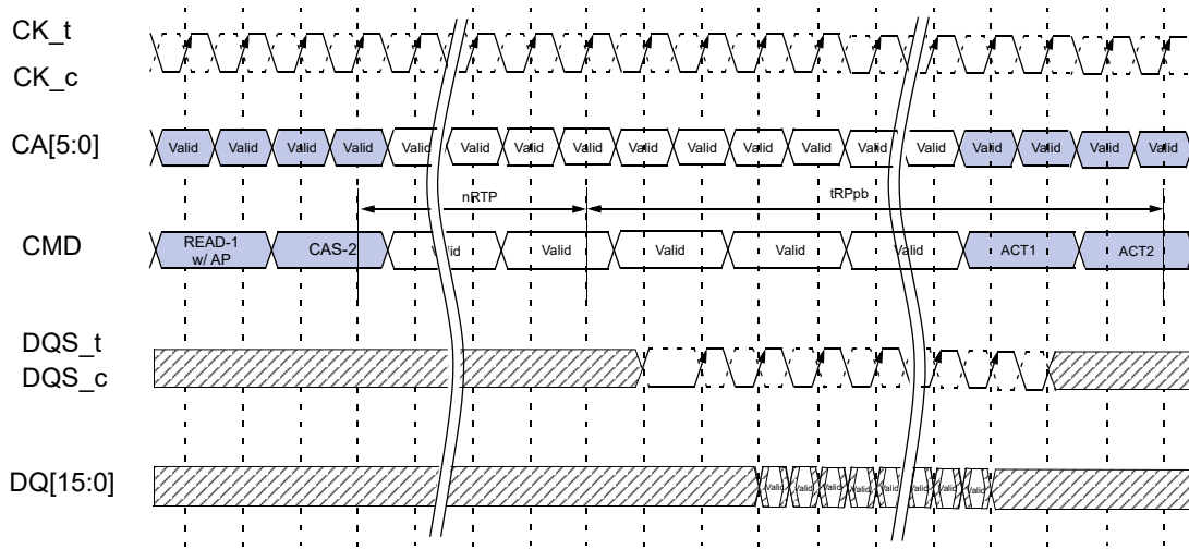
Figure - Burst Read with Auto-Precharge (BL16, Toggling preamble)
