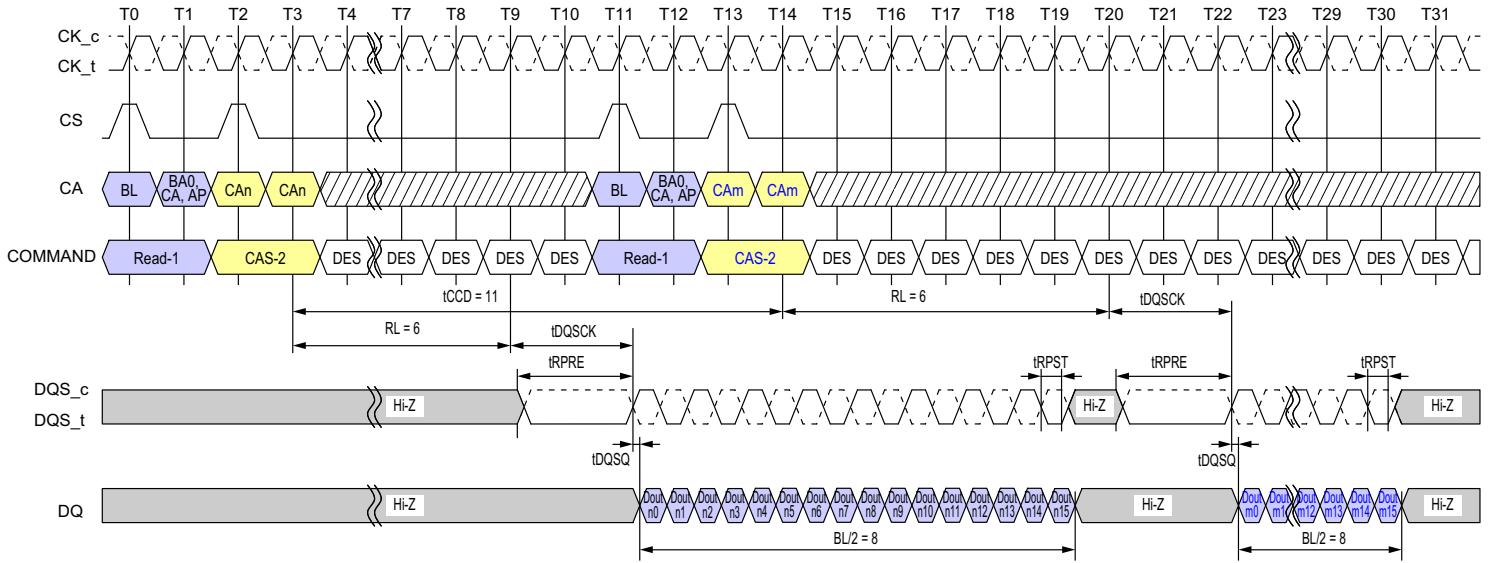
Figure - Consecutive Reads Operation: t_{CCD} = \text{Min} + 3 , Preamble = Static, 0.5nCK Postamble
