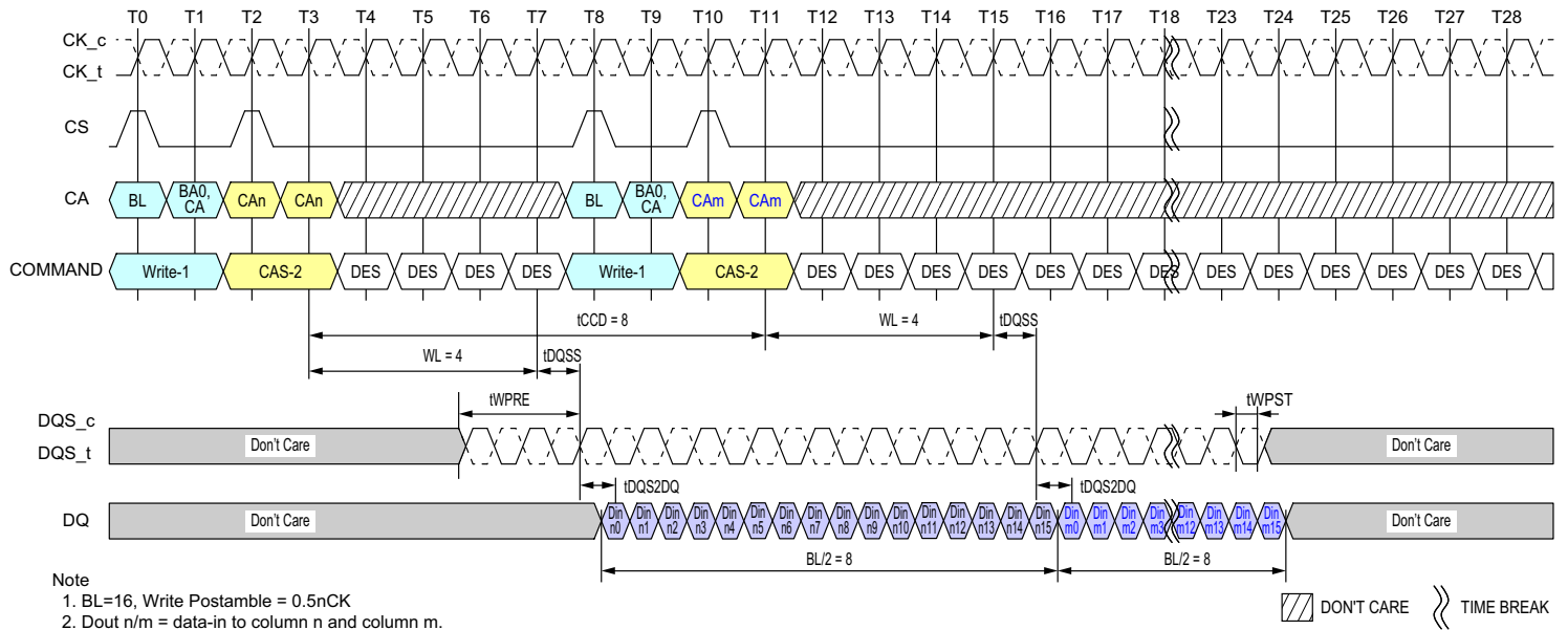
Figure - Seamless Writes Operation: t_{CCD} = \text{Min}, 0.5n\text{CK} Postamble
